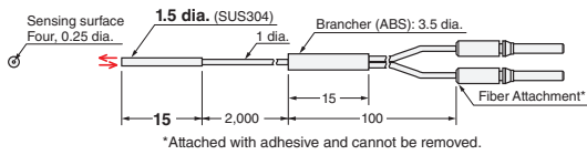
Enlarged View of Sensing Surface
