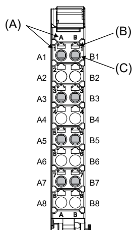
Eight-terminal Block
