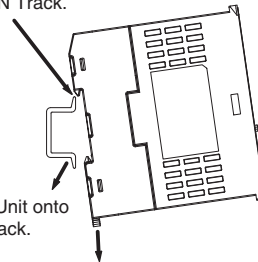
1. Pull down the hook.
