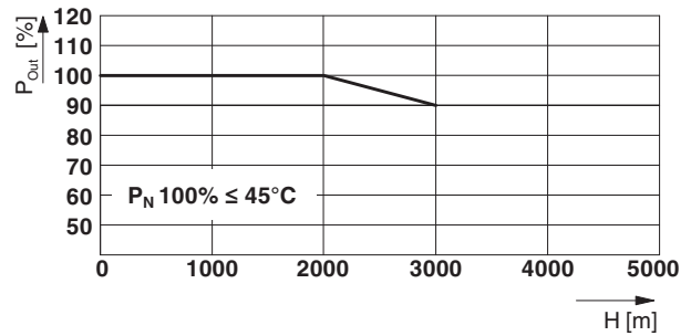
Figure 24 Output power depending on the installation height
