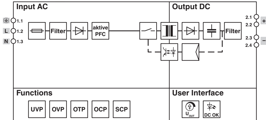
Figure 4 Block diagram
