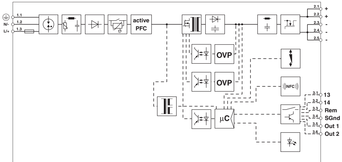
Figure 7 Block diagram
