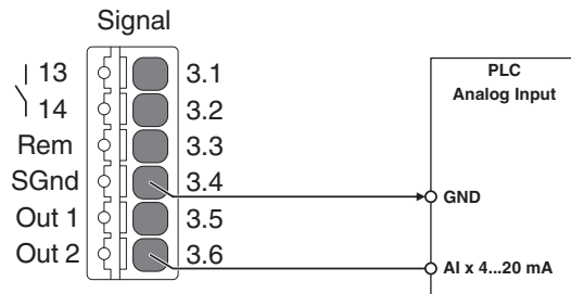
Figure 35 Signaling
