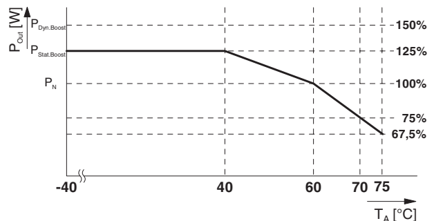
Figure 25 Performance characteristic in static boost
