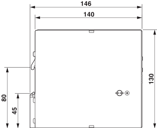
Figure 5 Device dimensions (dimensions in mm)
