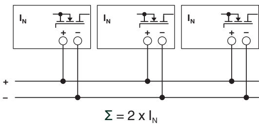
Figure 47 Schematic diagram, n+1 redundant operation for 80 A output current
