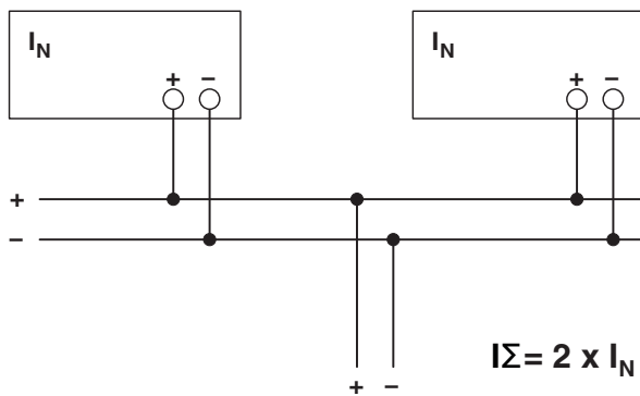
Figure 27 Schematic diagram of increased performance
