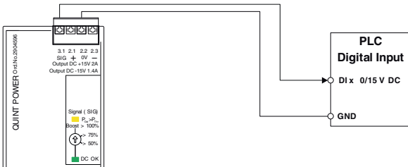
Figure 23 Signaling
