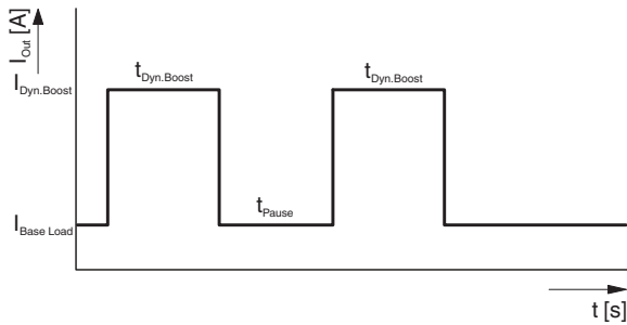
Figure 17 Basic curve of the dynamic boost process
