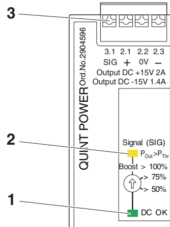
Figure 21 Position of signaling elements
