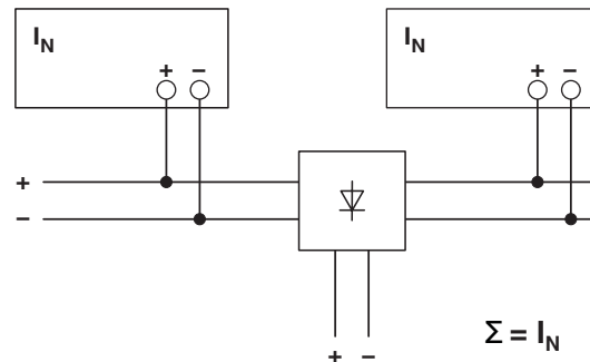
Figure 26 Schematic diagram, redundant operation with diode
