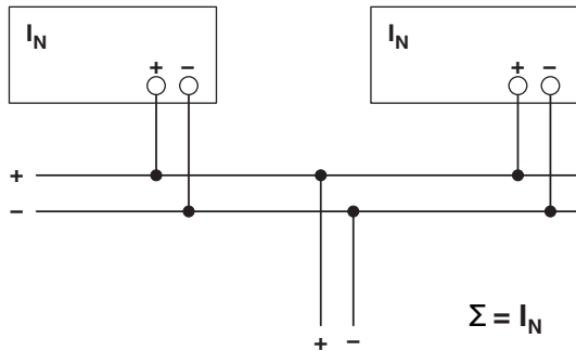
Figure 25 Schematic diagram in parallel operation
