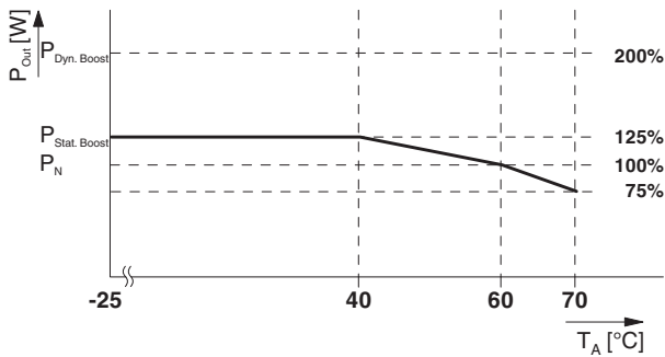
Figure 28 Output power depending on the ambient temperature
