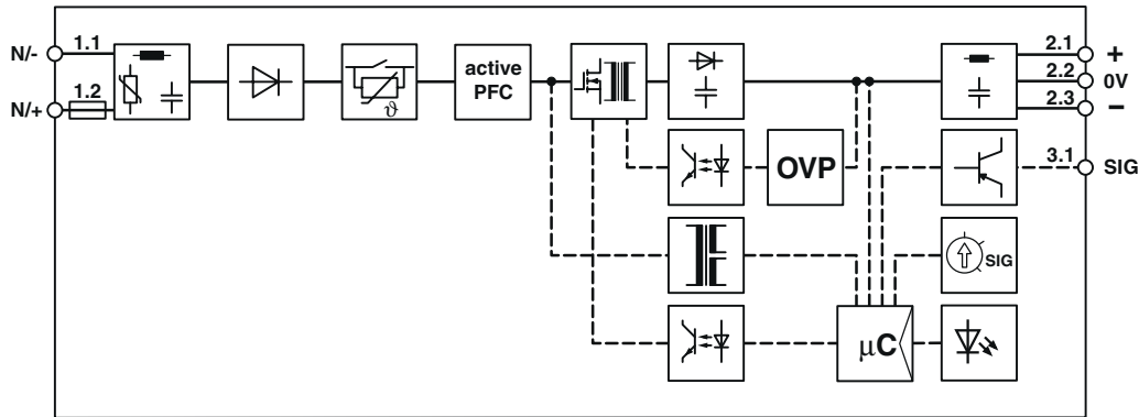
Figure 6 Block diagram
