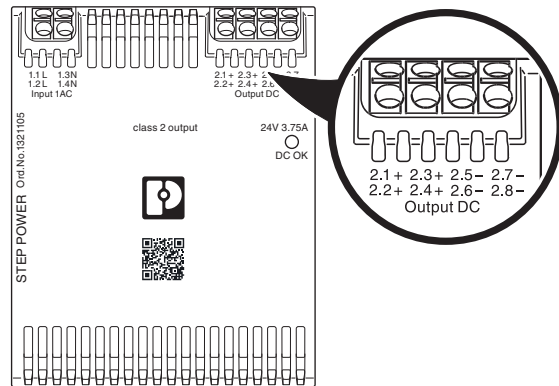
Figure 20 Position of DC output terminals
