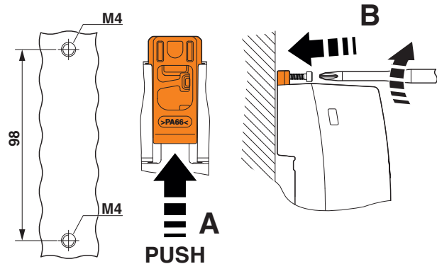
Figure 13 Screw fixing of the LED power supply to the mounting surface
