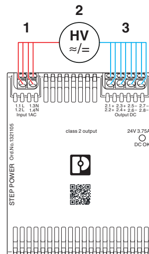
Figure 3 Potential-related wiring for the high-voltage test
