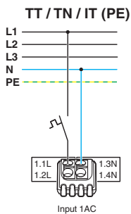
Figure 17 Schematic diagram, single-phase fuse protection
