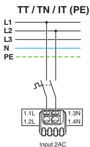
Figure 18 Schematic diagram, two-phase fuse protection
