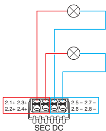
Figure 21 Wiring principle for DC output terminal blocks
