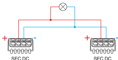
Figure 25 Schematic diagram, power increase in parallel operation
