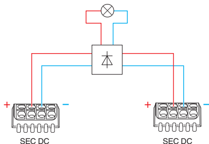
Figure 26 Schematic diagram, 1+1 redundancy with redundancy module (active or passive)
