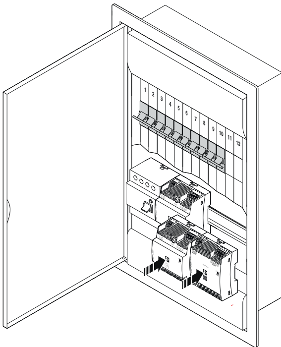
Figure 28 Schematic diagram, STEP POWER (4 HP) in a flush-mounted distributor (12 HP)
