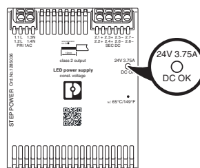
Figure 22 Position of DC OK LED
