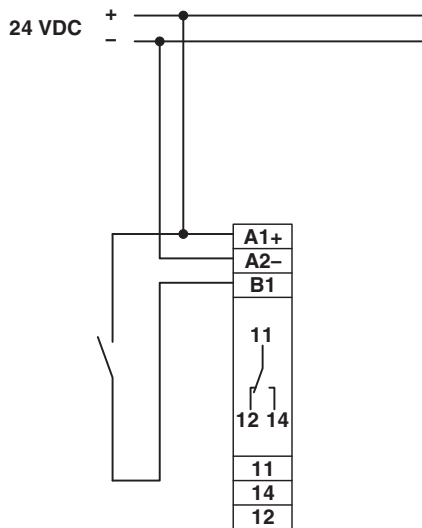
Figure 2 Connection with control contact
