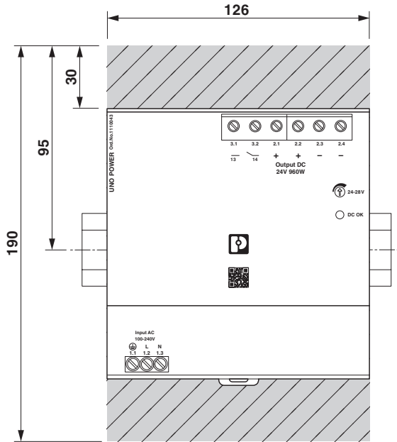
Figure 9 Device dimensions and minimum keep-out areas (in mm)
