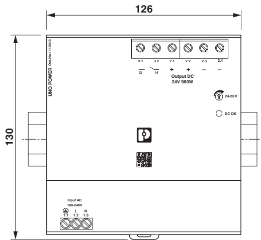
Figure 6 Device dimensions (dimensions in mm)
