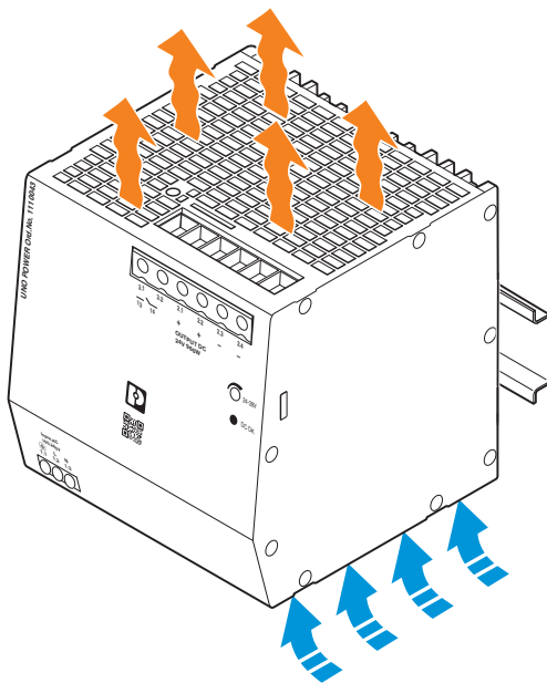
Figure 7 Schematic diagram of the convection cooling
