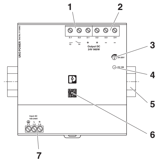
Figure 3 Location of functional elements and device connections
