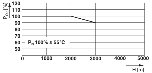
Figure 27 Output power depending on the installation height
