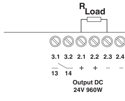
Figure 18 Wiring principle for DC output terminal blocks
