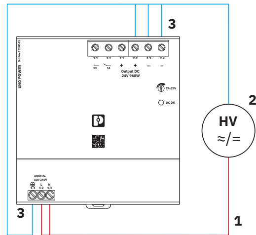
Figure 1 Potential-related wiring for the high-voltage test
